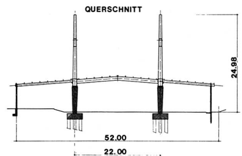
Fig. 3 Cross section
