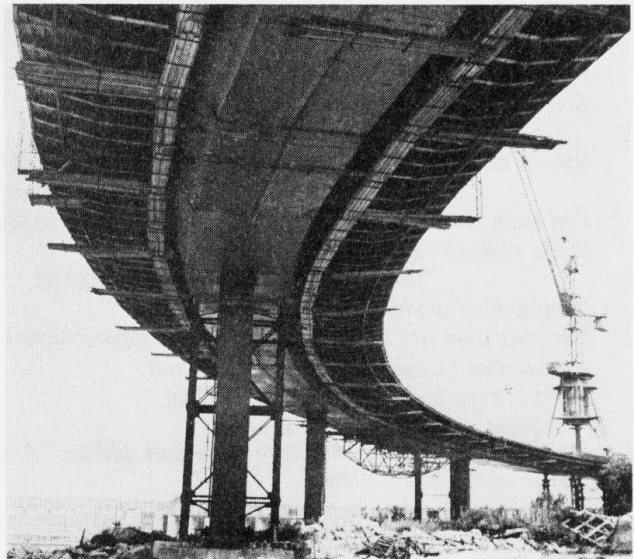
Fig. 4 General view of the bridge over ship-lock during the erection.
