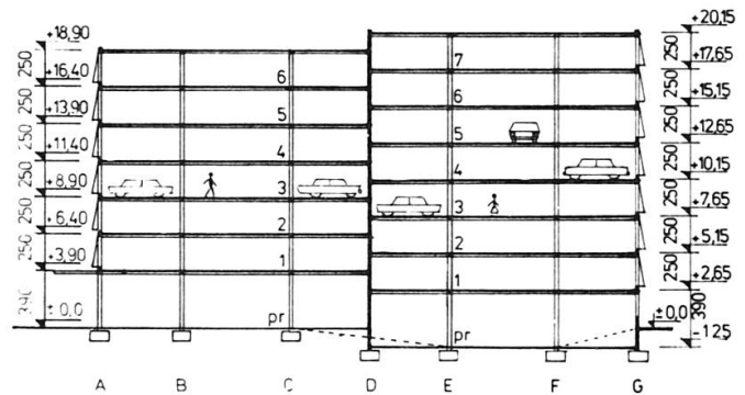
Fig. 3 Typical vertical section
