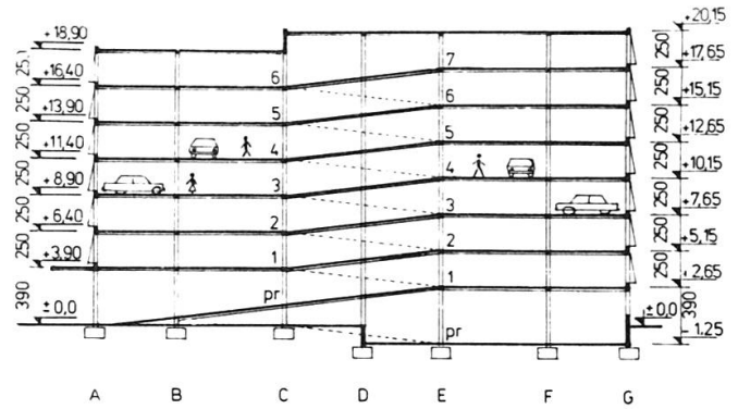
Fig. 2 Vertical section with the ramps
