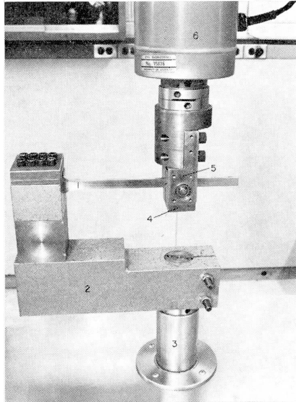
Fig. 7. Cantilever Beam Fixture.
