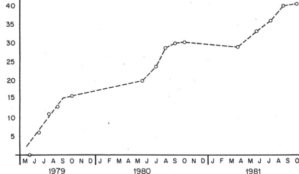
Figure 6. Radial geodetic displacements of P7.
