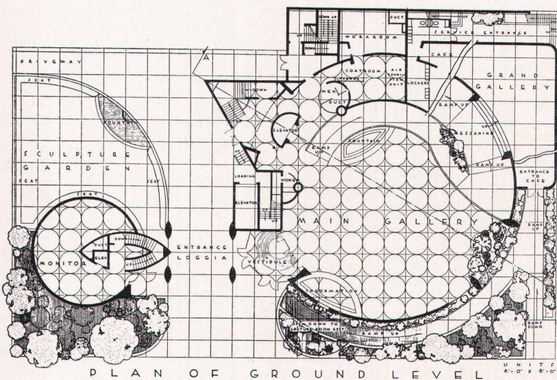
PLAN OF GROUND LEVEL UNIT 1: 600
