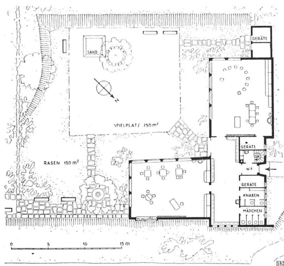
Abb. 48 Grundriß 1:300 | Plan | Ground floor
