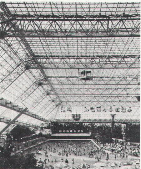
42 Summerland recreation center, Japan, 1975. Kinji Fukuda und Minoru Murakami
