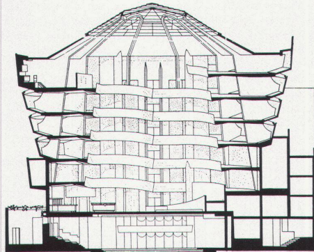
31 Solomon R. Guggenheim Museum, New York, 1956–1959. Frank Lloyd Wright
