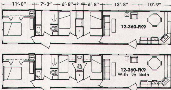
New 3 Bedroom Front Kitchen Floor Plan
