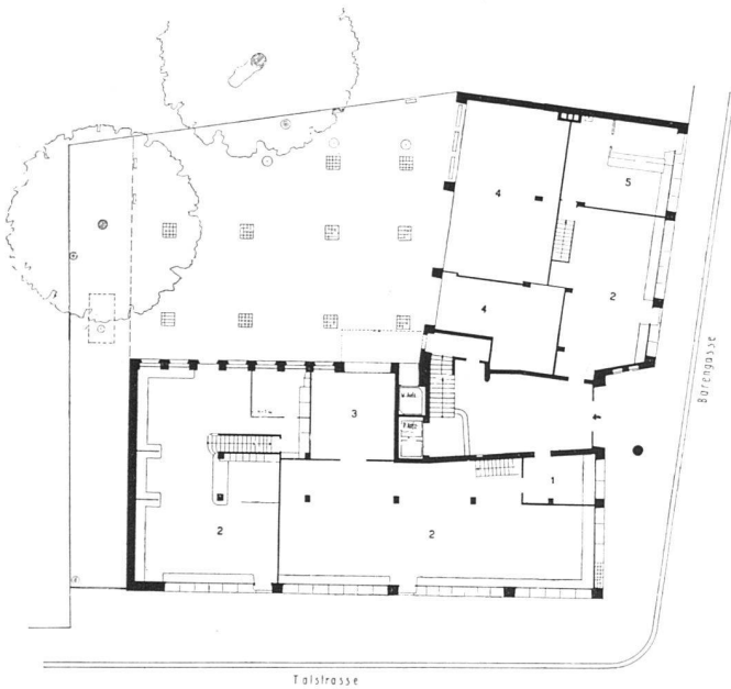
Erdgeschoß 1:500 | Rez-de-chaussée | Ground-floor
