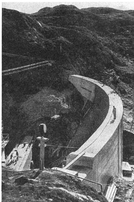
Staumauer Totensee
