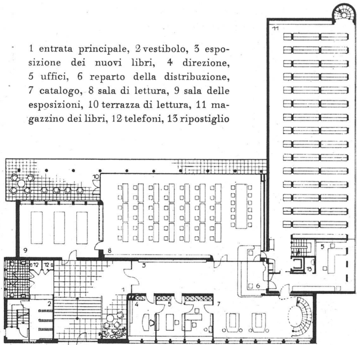
Piano terreno 1:400
