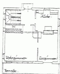
Erdgeschoss.
