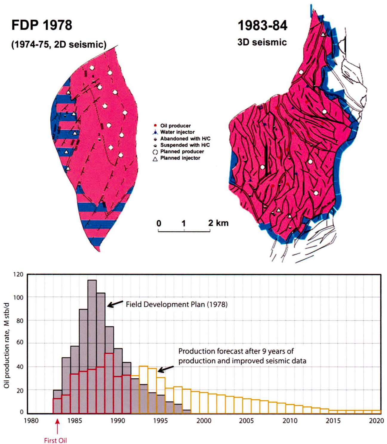
Fig. 1: The prediction capability of a geological model in support of any geo-energy resource development it is strongly depending on quality and amount of the subsurface data which almost by definition will be incomplete, discontinuous and often unreliable. Handling these uncertainties is therefore key for any sub-surface geo-model to be able to manage project risks. The first geological model of the Cormorant field (Northern North Sea, UK) based on few well penetrations and 2D seismic which was used to plan the field development plan (FDP) yielded a largely inaccurate production forecast which at that time did not take into account the possible complex reservoir compartmentalisation as it was revealed by the 3D seismic survey acquired in 1983-84 (modified after Lim 2002).
