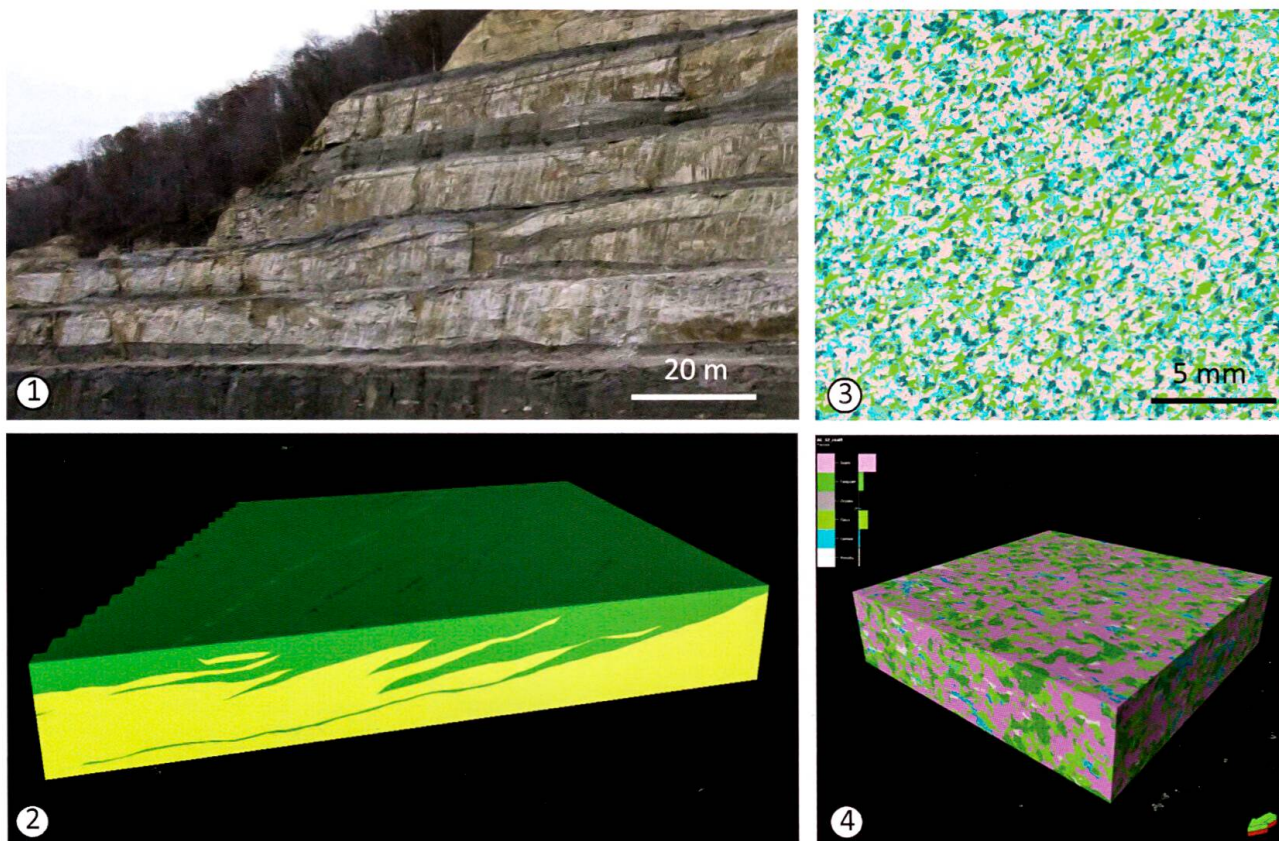
Fig. 9: Geo-modeling of different geological environments requires adequate tools able to capture their natural complexity. [1] Clinoform geometry at decameter scale from Upper Carboniferous fluvio-deltaic sandstones well exposed in Eastern Kentucky are modeled with a deterministic approach [2]. The microtexture of a sandstone reservoir [3], analysed by QEMSCAN quantitative automated petrography in two-dimensional environment (thin section) is modeled with multi-point statistics and the knowledge transferred in the three-dimensional space [4]. Modeling images courtesy of Aymeric Le Cottonnec, University of Geneva and Tatiana Chugunova, Total SA.
