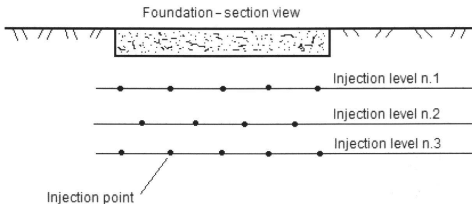
Fig. 3: Schematic representation of the Urettek injection procedure.
