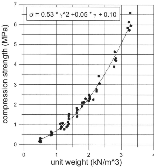
Fig. 1: Uniaxial compression test results: vertical stress \sigma vs. sample unit weight \gamma .
