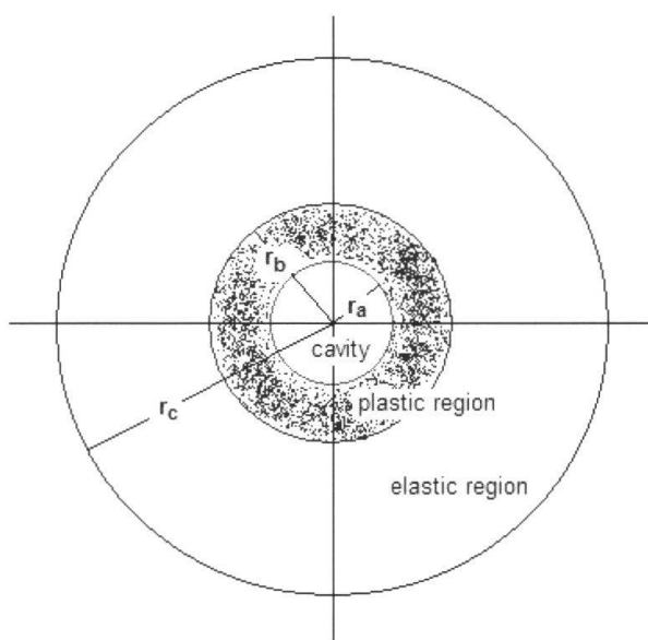
Fig. 4: Schematic representation of elastic and plastic zone surrounding the cavity.
