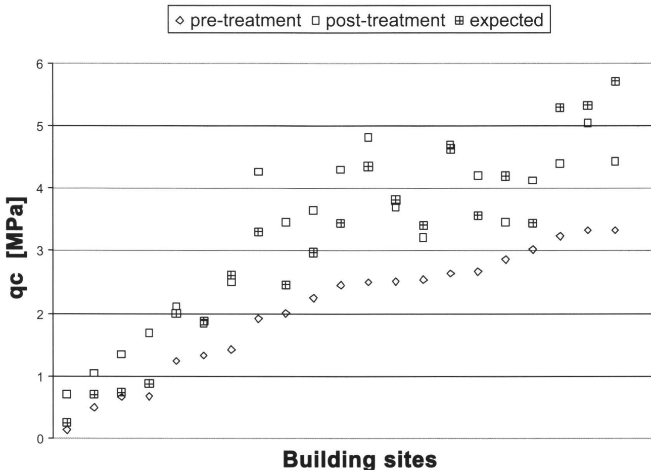
Fig. 7: Comparison among q_c values recorded before and after the ground improvement and calculated by an analytical model.
