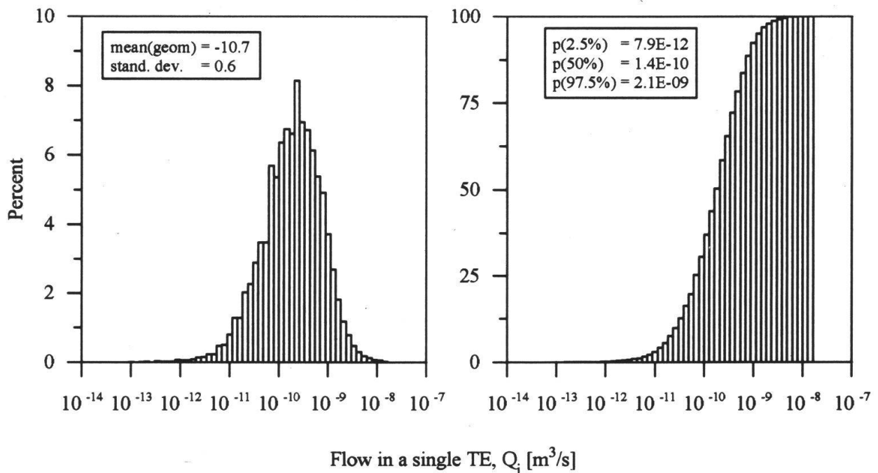
Fig. 6: Calculated distribution of volumetric flow in a single fracture, Q_i [ m^3/s ], full- and sparse scenario
