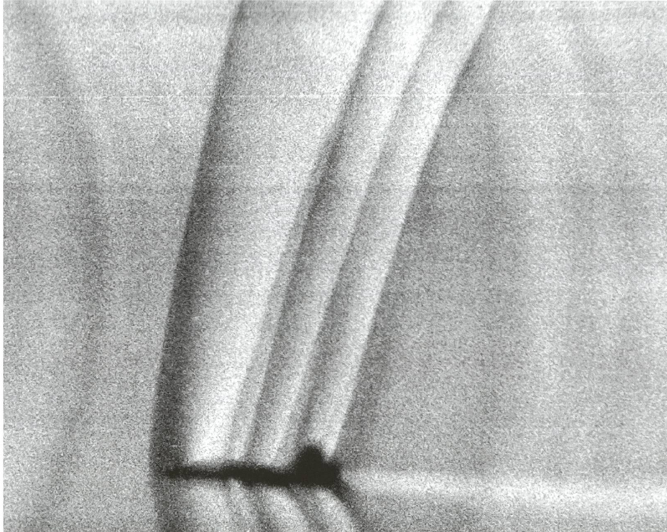
Schlieren photograph of T-38 shock waves at Mach 1.1, 13,000 feet [photo: Dr. Leonard Weinstein, 1993]
