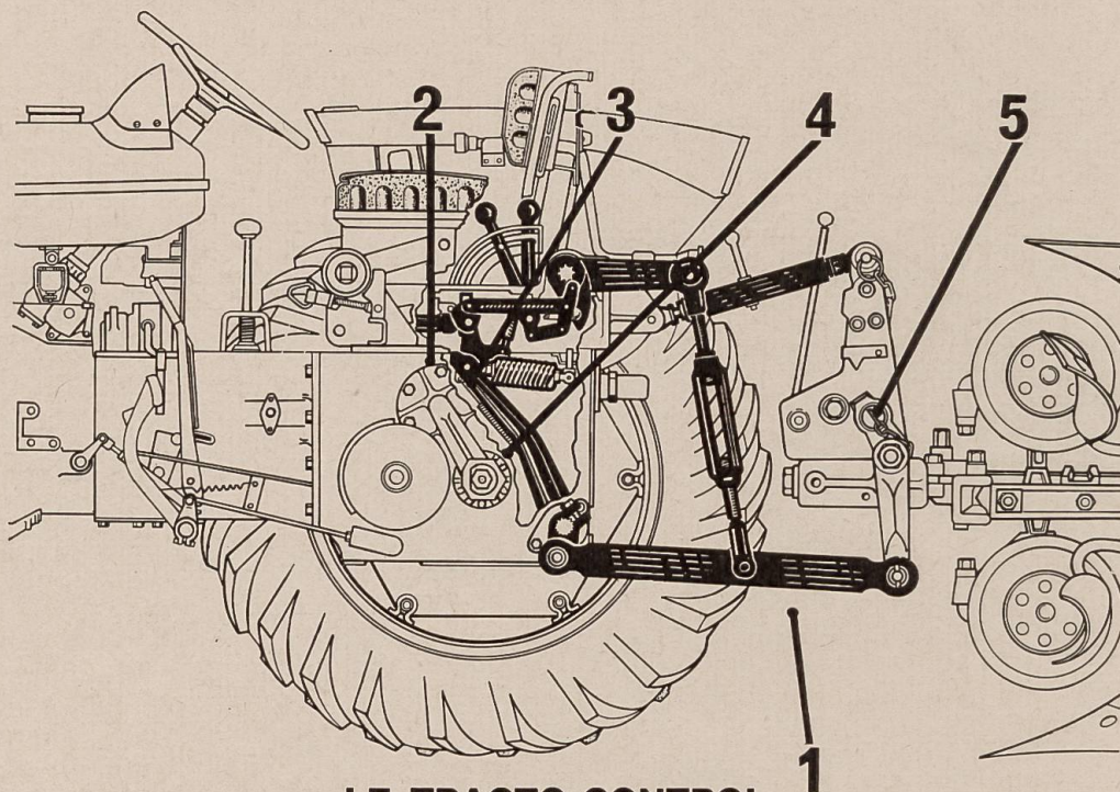
LE TRACTO-CONTROL
