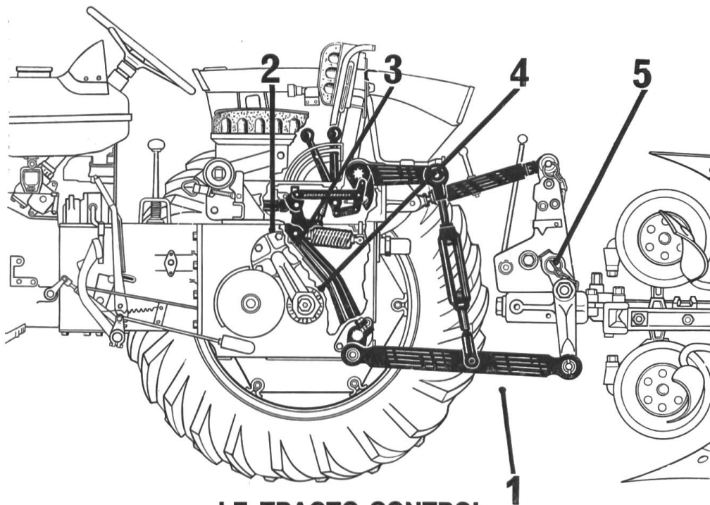
LE TRACTO-CONTROL
