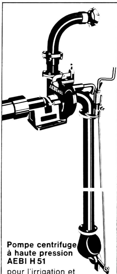
Pompe verticale
