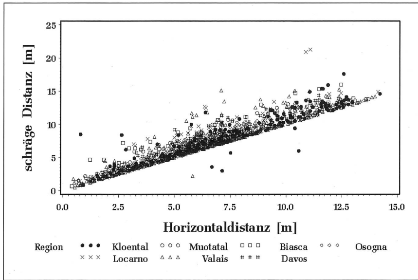
Abbildung 3: Horizontaldistanz versus schräge Distanz. Figure 3: Horizontal versus inclined distance.
