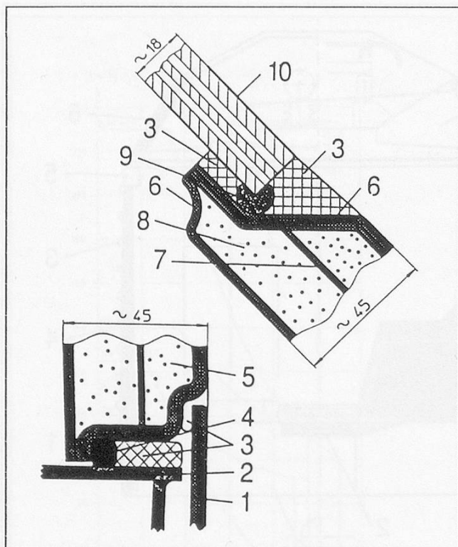
Figure 7: Assembly of driver's cab windows. Courtesy SLM
