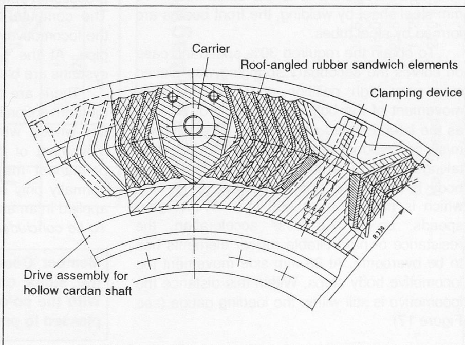
Figure 19: Flexring drive, sandwich elements. Courtesy SLM
