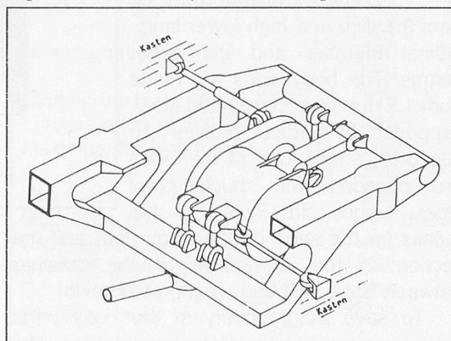
Figure 10: Drive unit support in bogie.
