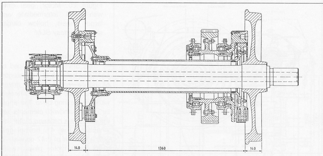
Figure 18: Flexring drive on wheelset. Courtesy SLM
