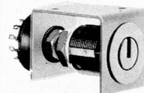
KS531. 3-pole 4 way 5 amps at 300 VAC/DC.
