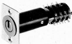
500 Series. Rotary wafer switch 5 amps at 300 VAC/DC.
