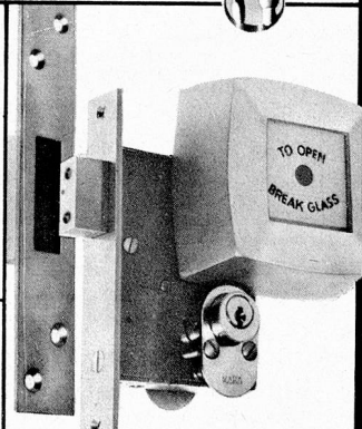
Emergency Exit Mortice Deadlock
