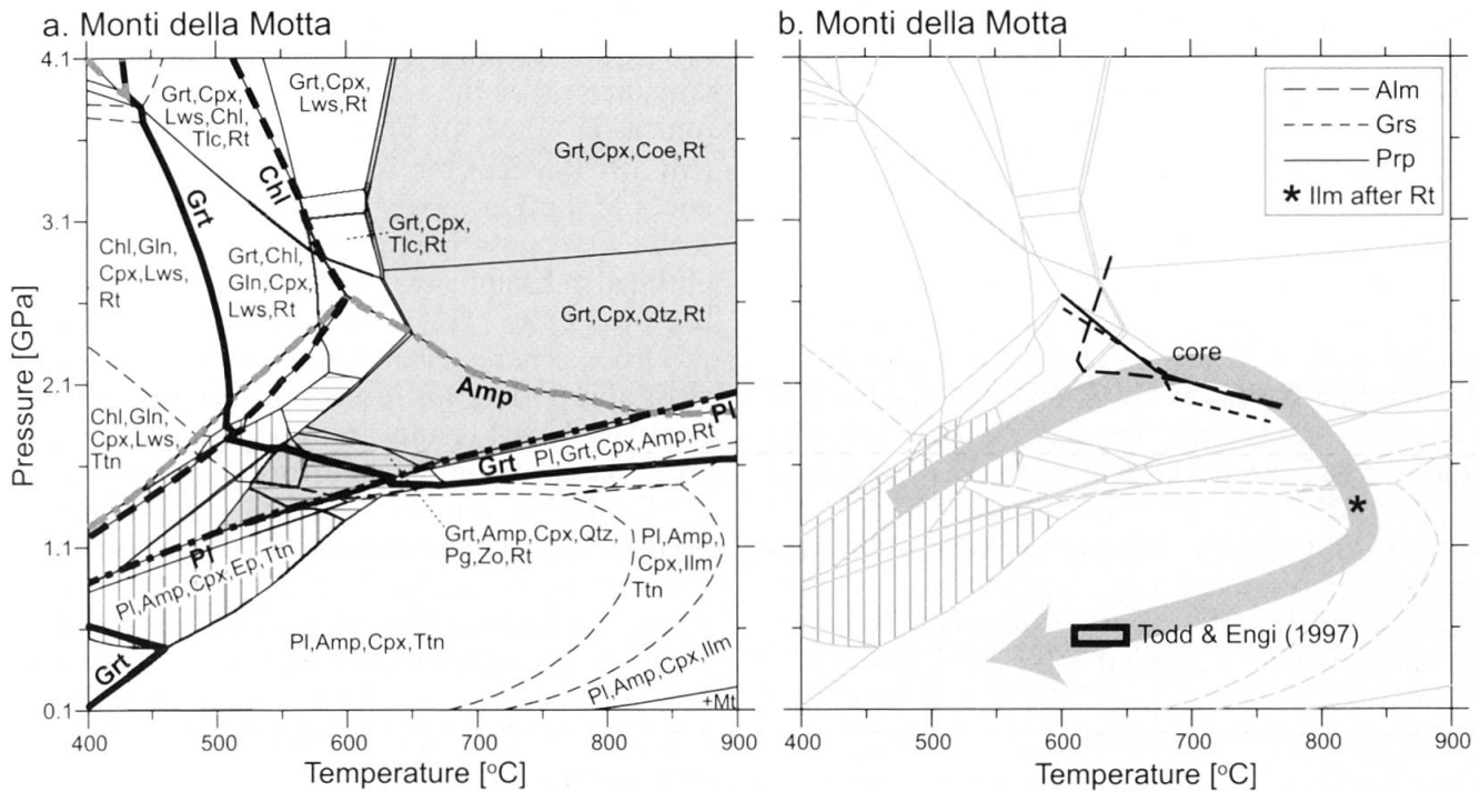
Fig. 15 (a) Computed phase relations for Monti della Motta sample Be9918 in the system CNFMASHTi, assuming fluid saturation and QFM-buffering. Grey shading indicates presence of quartz (very low modal abundance at eclogite conditions), horizontal stripes the presence of zoisite and vertical stripes denote epidote. Thick black line = garnet, black dash-dot line = plagioclase, grey dash-dot line = amphibole, thick black dashed line = chlorite, thin dashed lines = ilmenite-rutile-titanite. (b) Isopleths for garnet core composition calculated using DOMINO. Star marks the appearance of ilmenite after rutile and the black box indicate the PT conditions of the Barrovian overprint (Todd and Engi, 1997). Grey arrow indicates approximate PT-path for the sample.
