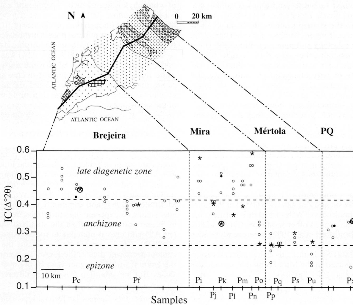
Fig. 3 Illite crystallinity (IC) of the studied samples, in relation to their geological and sample locations (*—sandstones, ○—metapelites). PQ—Phyllite-Quartzite Fm. Samples studied by TEM: circled *—sandstones; ●—metapelites). Data for metapelites are from ABAD et al. (2001).
