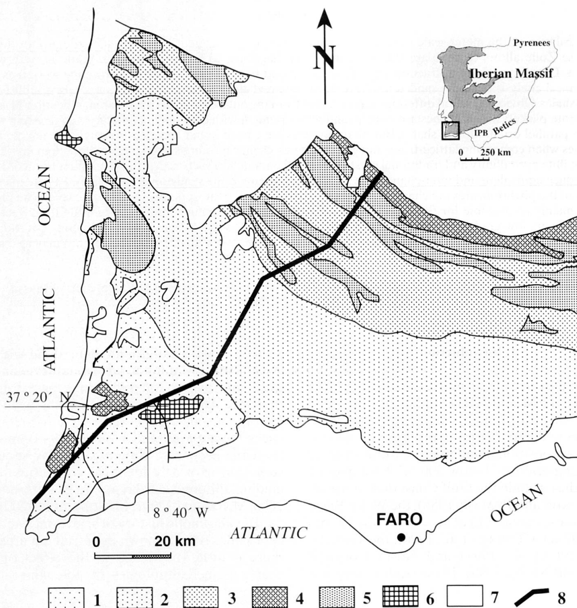
Fig. 1 Geological map of the South Portuguese Zone (adapted from OLIVEIRA, 1990 and QUESADA et al., 1991). Syn-orogenic flysch sequences of the Baixo Alentejo Flysch Group (Culm): 1—Brejeira Formation; 2—Mira Formation; 3—Mértola Formation; 4—Pre-orogenic sequences (mainly Phyllite-Quartzite Formation); 5—Volcano-Sedimentary Complex; 6—Peralkaline intrusions; 7—Meso-Cenozoic detrital cover; 8—Profile of sample location.
