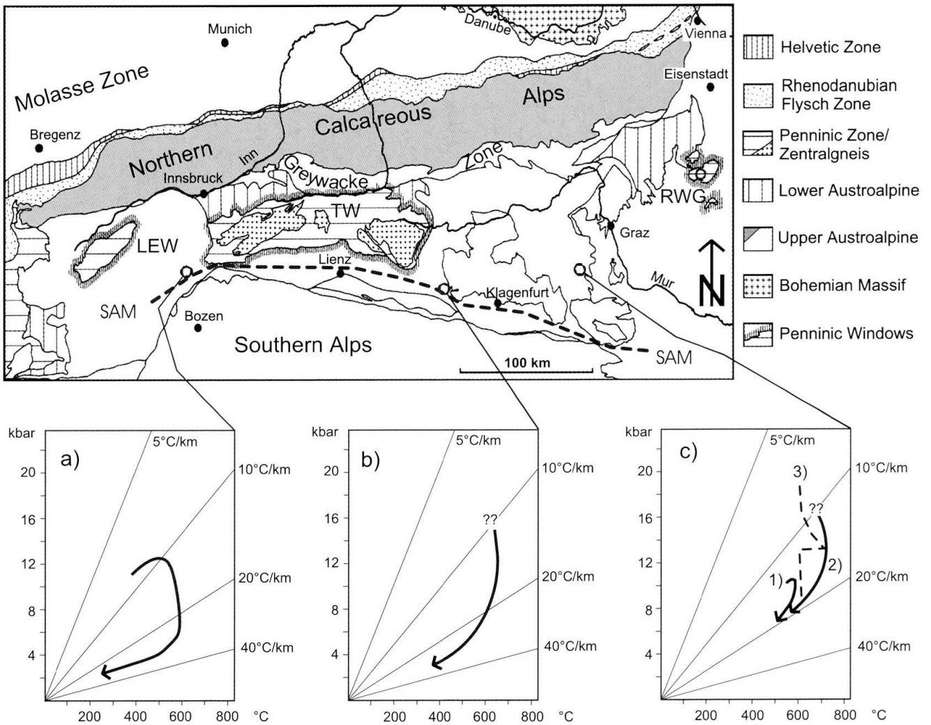
Fig. 2 Geological sketch map of the Eastern Alps and three characteristic PT paths for the a) Southern Ötztal basement (HOINKES et al., 1991), b) Millstatt basement (TEIML, 1996), c) Koralm: 1) Plankogel unit, 2) Koralm unit (GREGUREK et al., 1997); 3) Koralm "Plattengneis" (STÜWE and POWELL, 1995).
