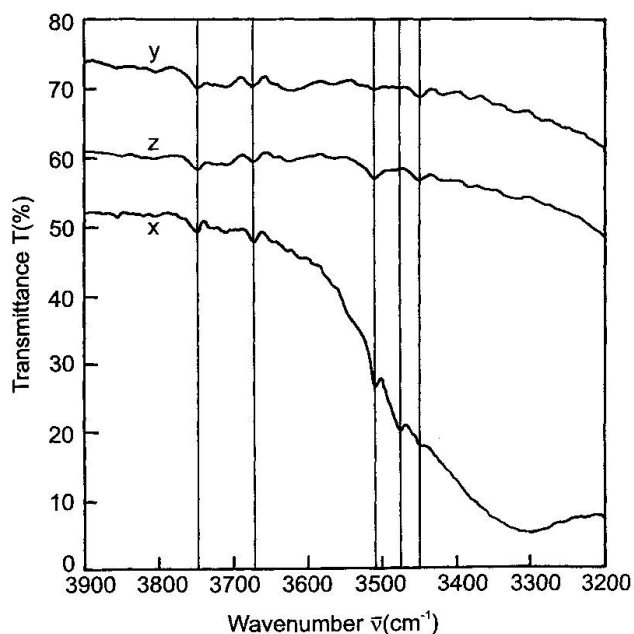
Fig. 2 Polarized FTIR spectra of oriented sinhalite single crystal sections (normalized thickness 1.0 cm). The x-spectrum ( \mathbf{E} vibrates parallel to [100] ) was measured on (010) and (001), the y-spectrum ( \mathbf{E} parallel [010] ) on (001) and the z-spectrum ( \mathbf{E} parallel [001] ) on (010). The vertical thin lines indicate maximum band positions at 3740 , 3670 , 3509 , 3474 and 3445\text{ cm}^{-1} .
