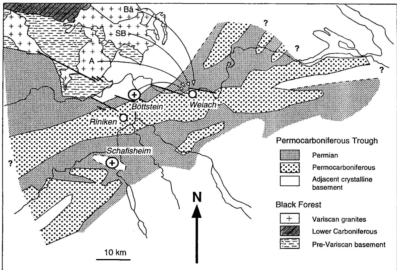
Fig. 1 Simplified tectonic map of the Permian Carboniferous Trough of Northern Switzerland and of Southeastern Black Forest; from THURY et al. (1988). The four NAGRA wells of Böttstein, Riniken, Schafisheim and Weiach are indicated. Detrital zircons in Upper Carboniferous clastic sediments may be traced to the granites of Bärhalde (Bä), St. Blasien (SB), Albtal (A), Schafisheim or Böttstein, see text.
