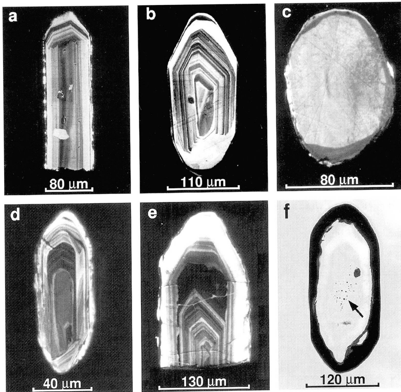
Fig. 1 a–e Cathodoluminescence images of representative zircons of the samples studied. Euhedral zircons from gabbroic eclogites Gi55 ( a ), Gi69 ( b ) and Zg1 ( d , zircon extracted from garnet; e , zircon from rock matrix) show multiple magmatic zoning, in contrast to the anhedral zircons from basaltic eclogite Ua0 ( c ) which are characterized by homogenous interiors and coarse marginal zonation. ( f ) Transmitted-light micrograph of zircon from sample Zg1 (matrix) showing "bubble core" structure (dark dots marked by arrow) indicative of inheritance.
