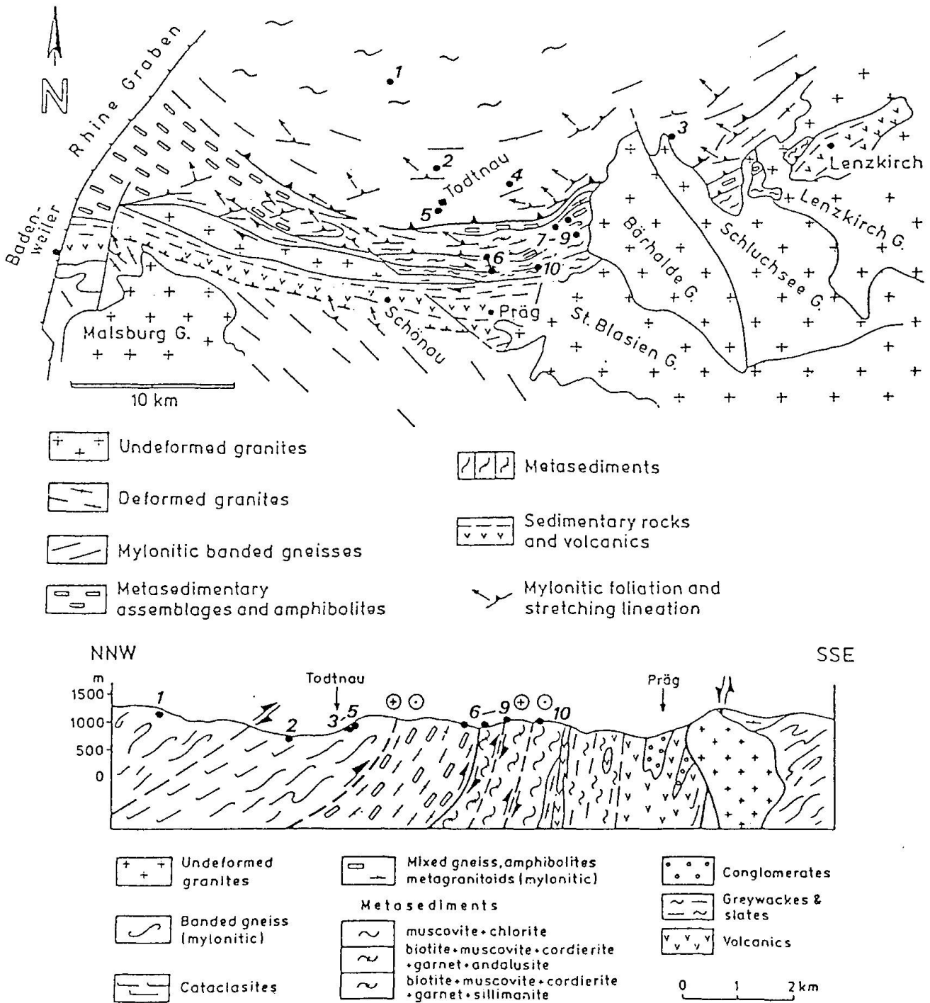
Fig. 4 Geological sketch map and cross-section through the oblique thrust and metamorphic gradients between the southern CGC and the Badenweiler-Lenzkirch Zone and stops (modified after KROHE and EISBACHER, 1988).
