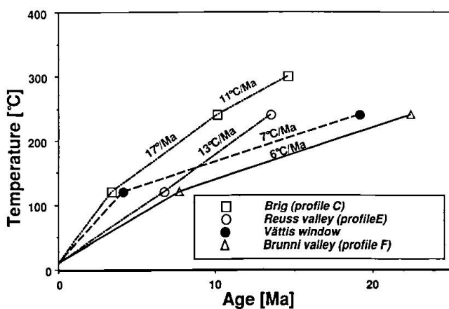
Fig. 11 Cooling curve from the Brig region based on the different blocking temperatures. K-Ar biotite age from PURDY and JÄGER (1976).
