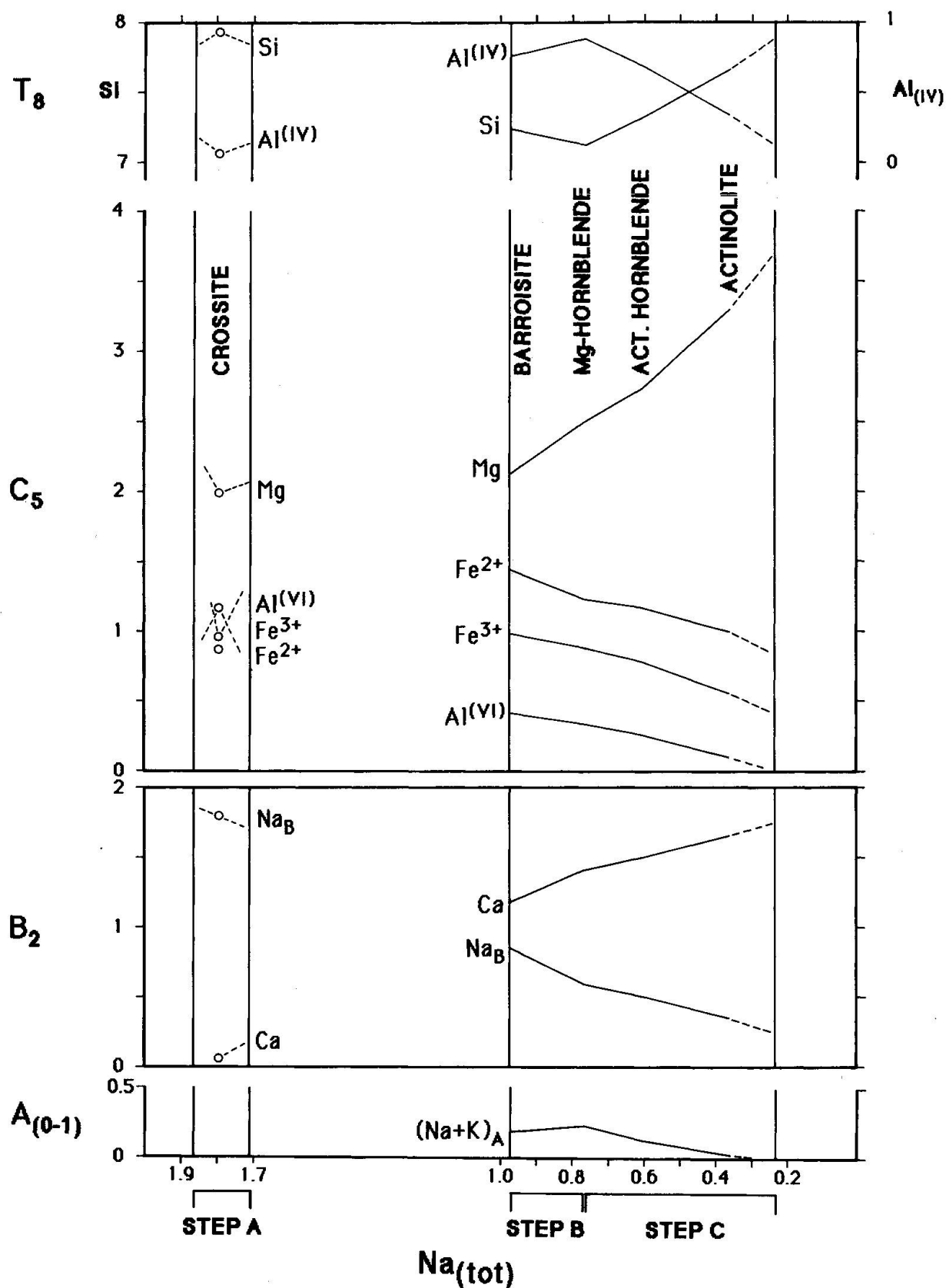
Fig. 5 Compositional trends in amphiboles: A_{0-1} B_2 C_5 T_8 O_{22} (OH)_{22} , plotted against \text{Na}_{(\text{tot})} with respect to structural sites. Steps A, B and C indicate ranges of analysed \text{Na}_{(\text{tot})} -values with different compositional trends. Note the gap between crossite and barroisite.
