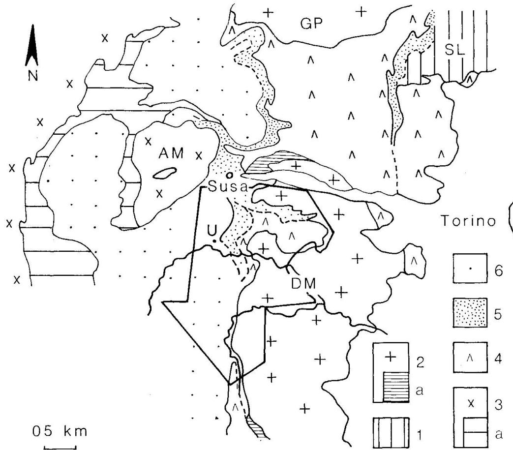
Fig. 1 Tectonic sketch map of the internal Western Alps. DM = Dora Maira, GP = Gran Paradiso, AM = Ambin massif, U = Usseaux.
