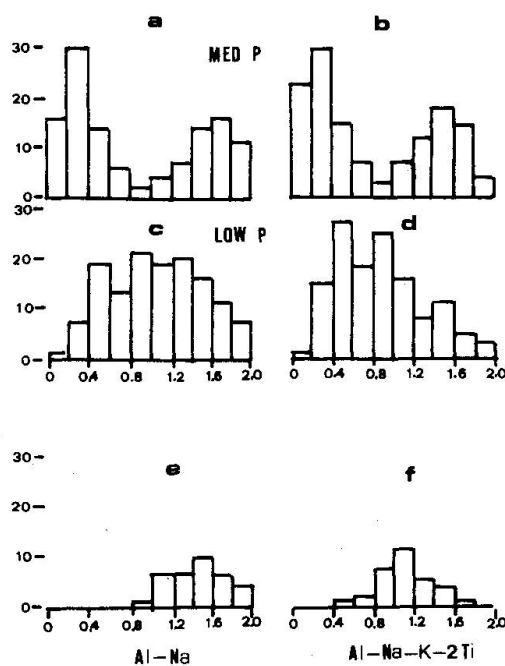
Fig. 5 Histograms of (Al-Na) and (Al-Na-K-2Ti) for medium- and low-pressure amphiboles. (a, b, c, d) after HYNES (1982) and our amphiboles (e, f). Data normalization to 23 oxygens with all iron as \text{Fe}^{2+} .
