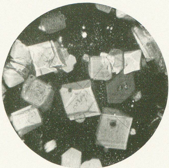
\text{Ca}(\text{NO}_3)_2 \cdot 2 \text{H}_2\text{O}
