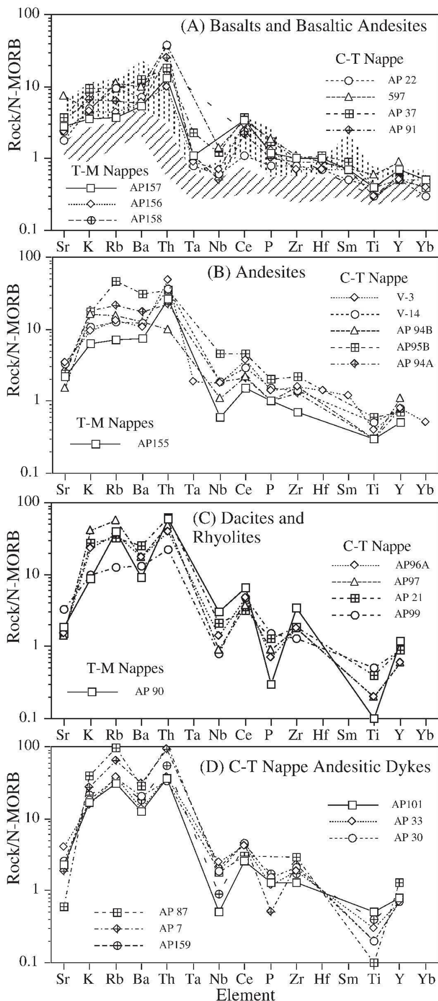
Fig. 4 Rock/N-MORB in-compatible elements diagrams for selected Jurassic volcanic and subvolcanic calc-alkaline rocks from SAM. Normalisation values and compositions of typical island arc basalts are from Pearce (1983). Hatched field: calc-alkaline basalts; dashed field: tholeiitic basalts.
