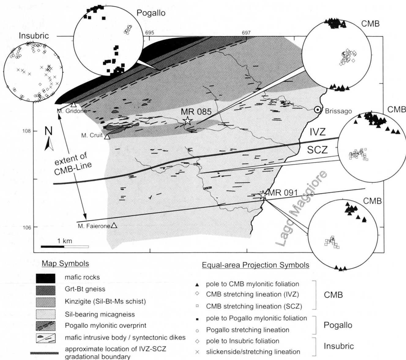
Fig. 2 Structural map of the Brissago segment of the CMB Line and the inferred contact of the IVZ and SCZ marked by a significant change in stretching lineations (after MULCH, 1999). Swiss topographic map grid coordinates are given for reference.
