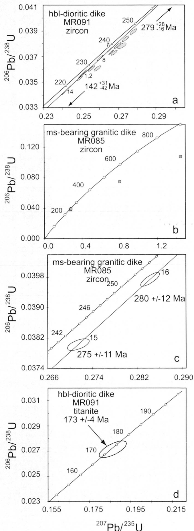
← Fig. 4 (a) U-Pb concordia diagrams of zircons from hornblende dioritic enclaves in syntectonic composite (MR091) and (b, c) granitic (MR085) dikes at the CMB Line. Note that analyses 15 and 16 in (c) fall onto the discordia line calculated in (a) for zircons from the composite dike (MR091) (calculated using analyses 1, 2, 6, 8, and 14) which is plotted for comparison only. (d) U-Pb concordia diagram for metamorphic titanite from syntectonic Early Permian composite dike (MR091). Ellipses indicate 2\sigma error.
