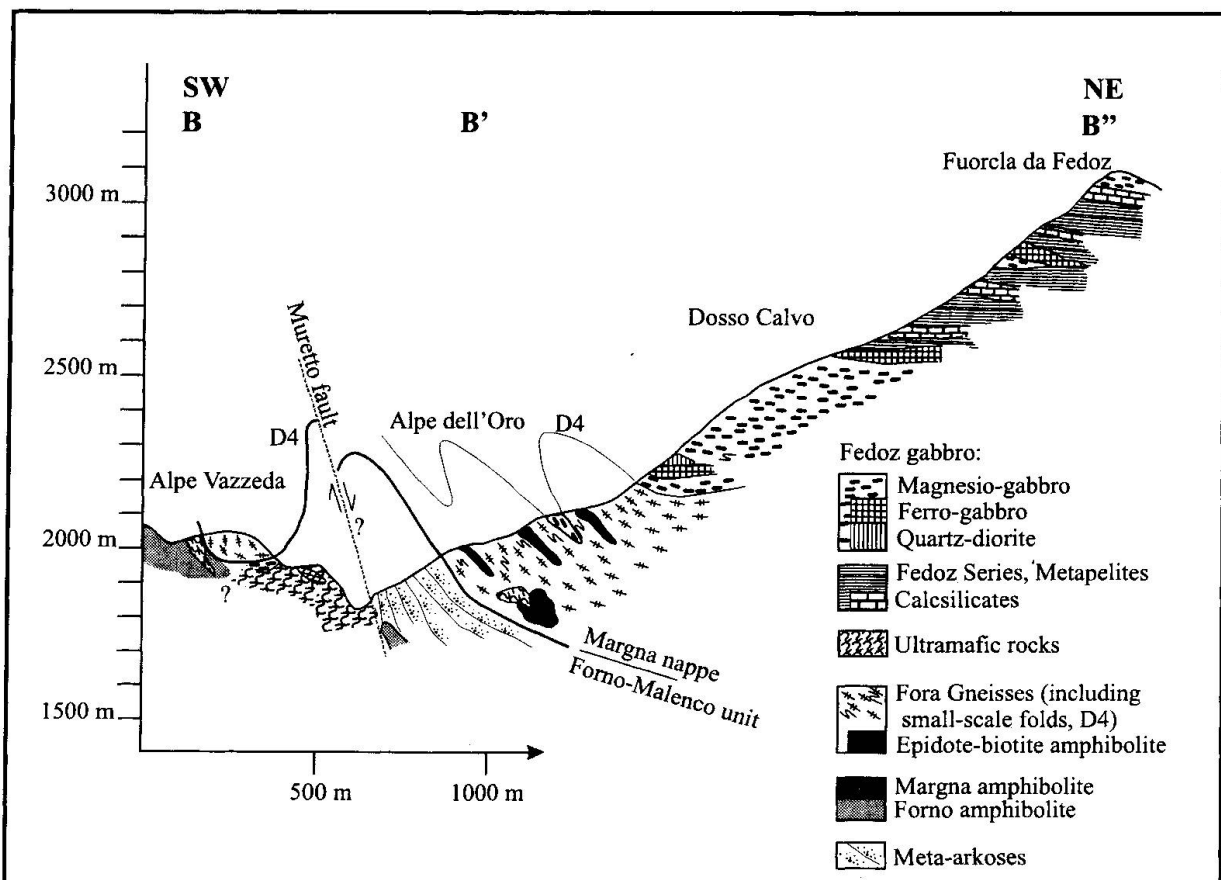
Fig. 6 Profile B-B'-B'' across the Val Muretto; for trace see figure 5. The D1-foliation is indicated by the orientation of the pattern, D4-folds have been outlined.
