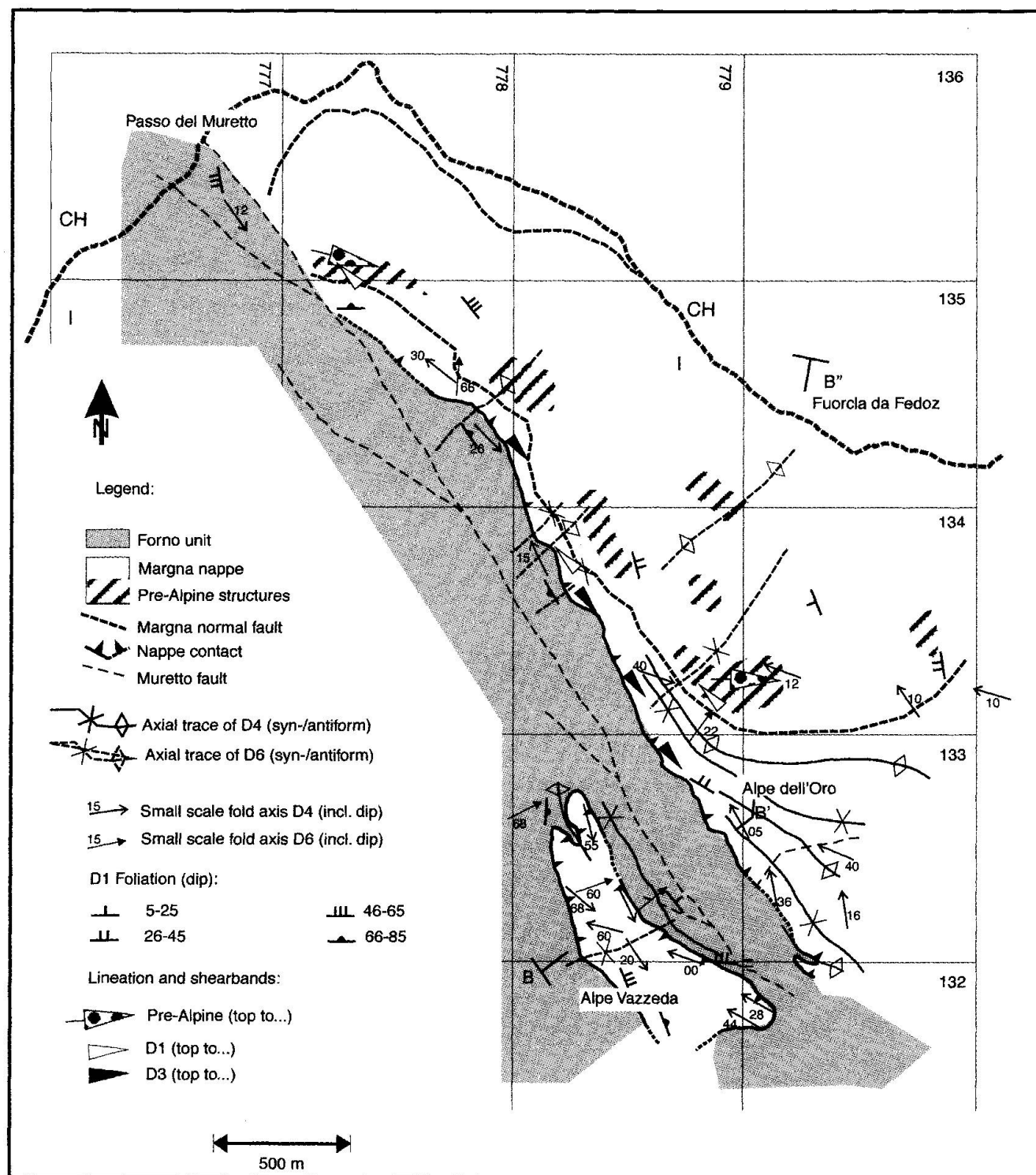
Fig. 5 Structural map of the Val Muretto. The Margna-klippe at Alpe Vazzeda can be explained by a basin structure due to overprinting D4 and D6 synclines (see Fig. 6).
