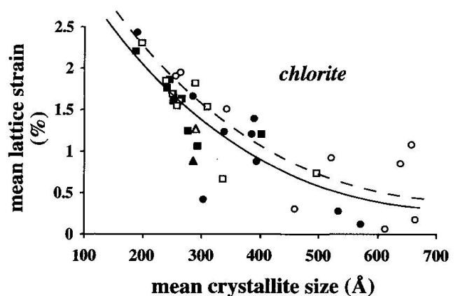
Fig. 10 Apparent mean lattice strain versus mean crystallite size of chlorite. For legend see the caption of figure 5.
