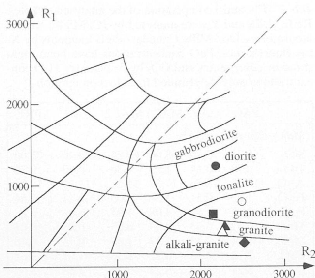
Fig. 2 Cumulative R_1 - R_2 diagram (DE LA ROCHE et al., 1980) for the analyzed granitoids. Symbols: ■ = polymetamorphic granodioritic augengneiss (PAG); ♦ = Cavour leucocratic metagranite (CAV); △ = Freidour metagranite (FRE); ● = porphyritic monzogranite of the Sangone Valley (SAN); ● = dioritic gneiss (MAL1) belonging to the "Malanaggio Diorite"; ○ = metagranodiorite (MAL2) belonging to the "Malanaggio Diorite".
