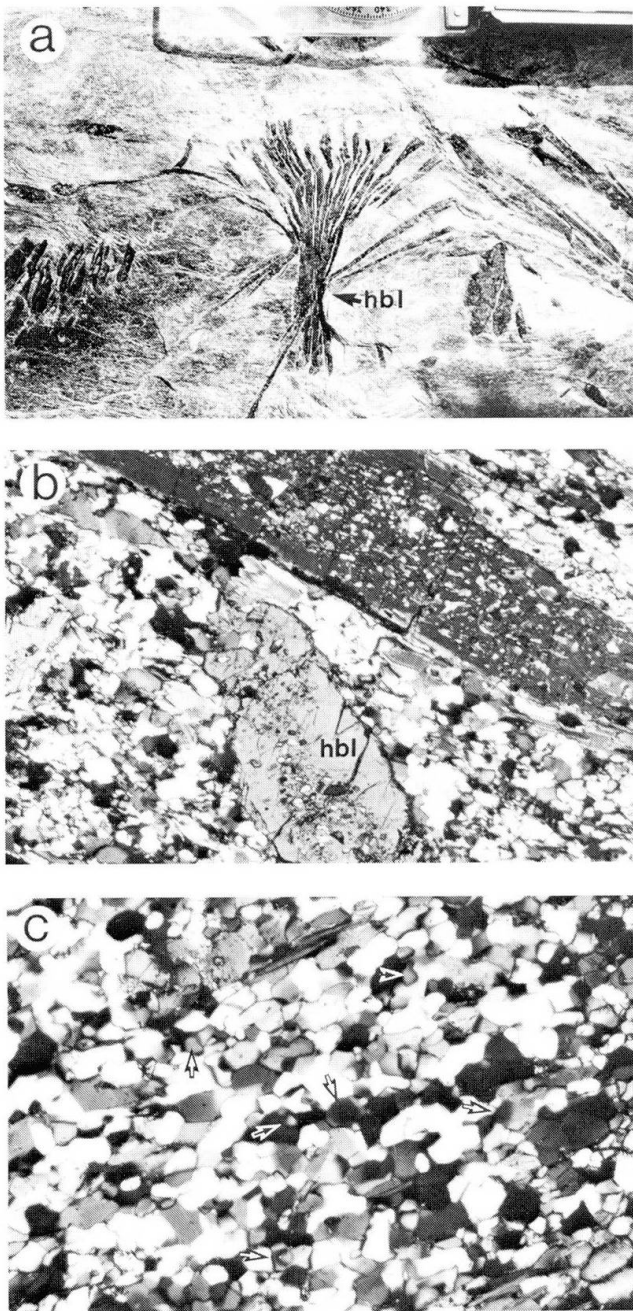
Fig. 4 (a) Typical outcrop appearance of hornblende garbenschiefer showing radiating spray of hornblende crystals. (b) Photomicrograph of hornblende garben in matrix of plagioclase and quartz; note grain coarsening indicated by change in grain size between plagioclase inclusions in hornblende and plagioclase in the matrix. Long dimension is 4 mm. (c) Detail of plagioclase-rich matrix showing asymmetric compositional zoning of grains (several indicated by arrows). Long dimension is 2 mm.
