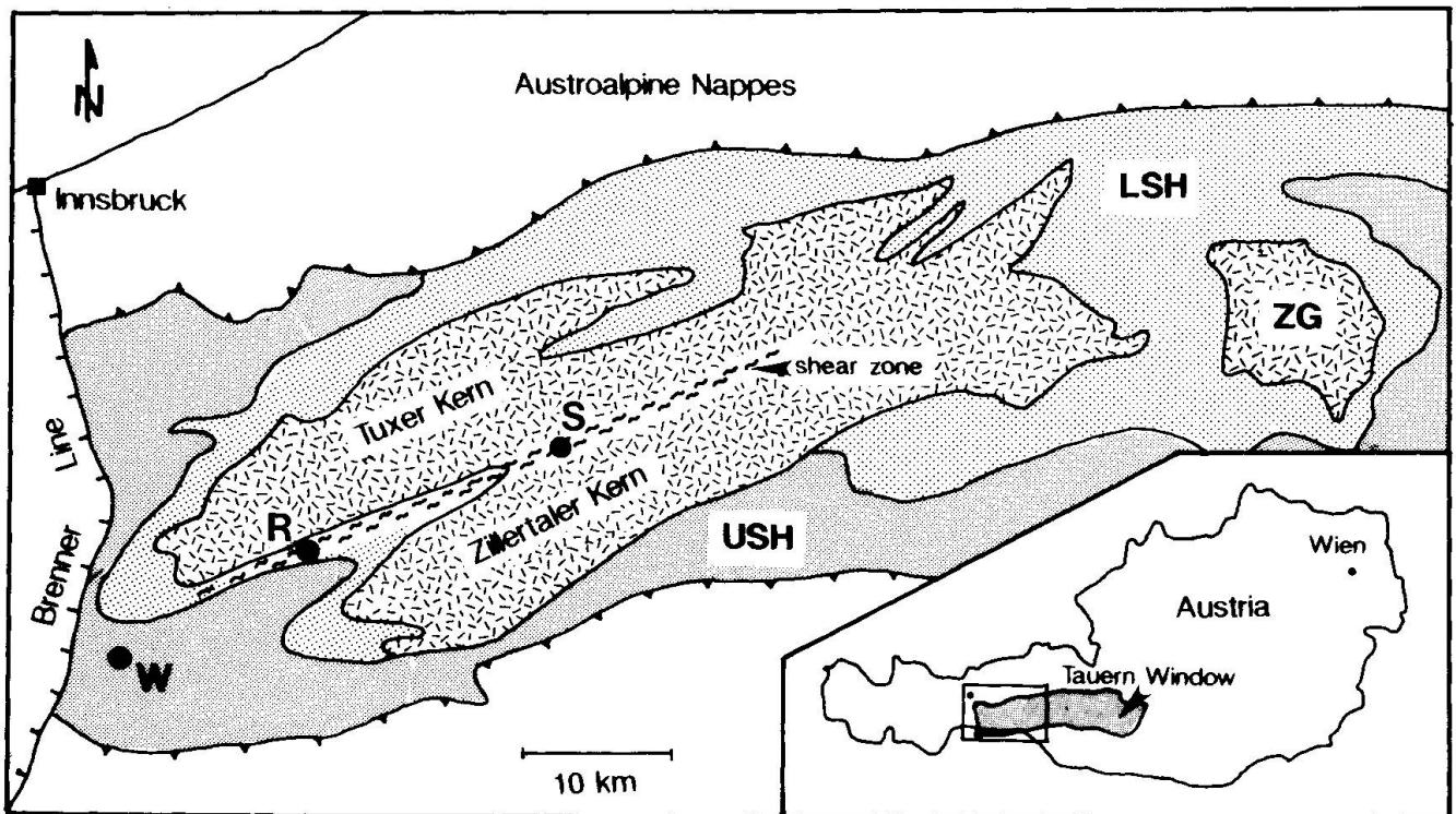
Fig. 1 Simplified geologic map of the western and central parts of the Tauern Window. ZG = Zentralgneis, which is divided into the granodioritic Tuxer Kern and tonalitic Zillertaler Kern in the west. LSH = Lower Schieferhülle; USH = Upper Schieferhülle. Brenner Line is a low-angle normal fault that unroofed the western part of the window in the Miocene. S = Stillup Tal; R = Rotbachlspitze; W = Weißspitze, which is a small klippe of Austroalpine material juxtaposed against the USH by the Brenner Line.
