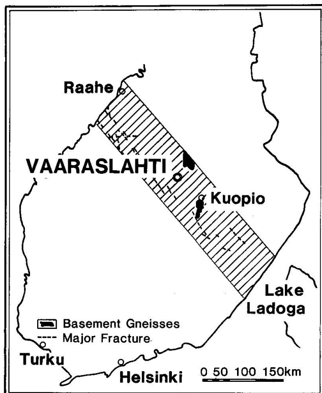
Fig. 1 Sketchmap of Southern Finland showing the location of Vaaraslahti within the main sulphide ore-belt running from northwest to southeast between Raahé and Lake Ladoga (after NEUVONEN et al. , 1981).
