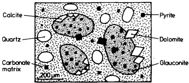
Fig. 2 Microscope observation in thin-section of a strongly lithified sample (e.g. Hauterivian).
