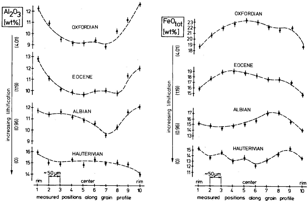
Fig. 6 Influence of lithification on Al_2O_3 and FeO_{tot} concentration. Numbers in parentheses represent the porosity in equivalent surface [ m^2/g sample].
