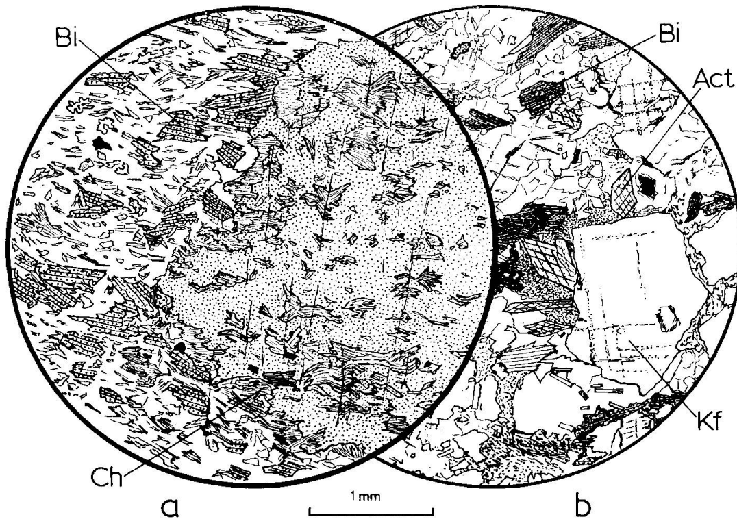
Fig. 9. a, Thin-section drawing of chiasolite hornfels with altered chiasolite porphyroblast, chlorite, biotite and a later cleavage. b, metamorphic arkose from the Sandstone Member with potash feldspar (Kf), actinolite, biotite, quartz and titanite.
