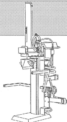
Hydro-Combi 10/20/30 t
