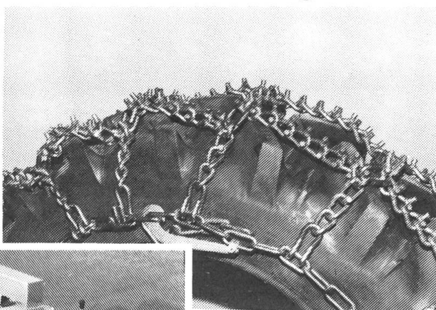
Trygg-Stollenkette
