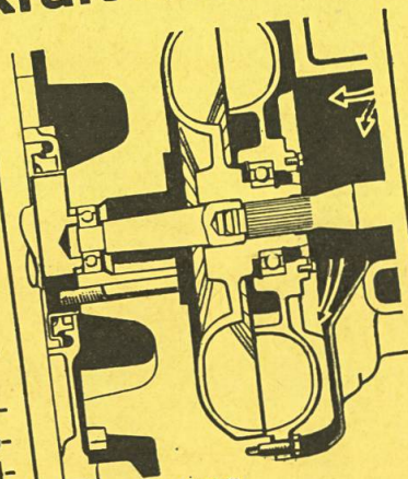
Turbokupplung
