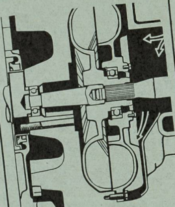
Turbokupplung
