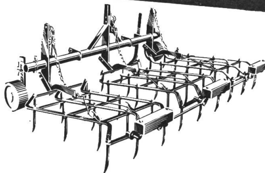
Ackeregge
